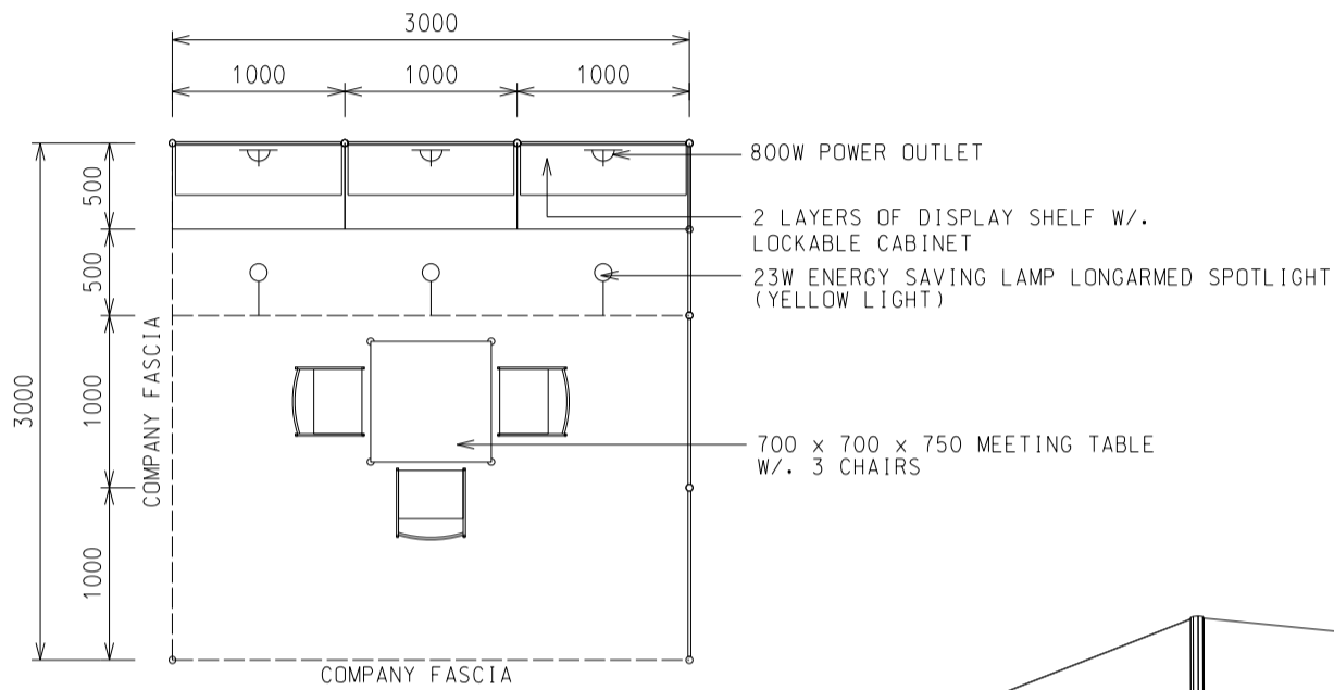
PLAN 3M(W) X 3M(D) X 2.5M(H) Left Corner Booth A
